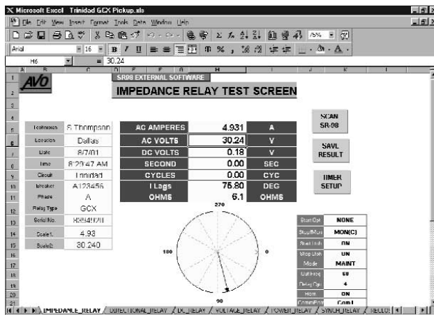
Shown above is a Test Screen for an Impedance Relay. The test result is for a Reach Test on a Impedance relay. The relay operated at 6.1 Ohms at a max torque angle of 75.8 degrees. The SR-98 software operates with Windows Excel version 7.0 or higher running under Windows 95/98/2000/NT or XP. Microsoft Excel, Microsoft Word, Windows 95, Windows 98, Windows 2000, NT or XP are all registered trademarks of Microsoft Corporation.
