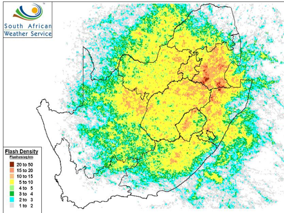
Lightning Flash Density Map for 1 January to 31 December 2007
