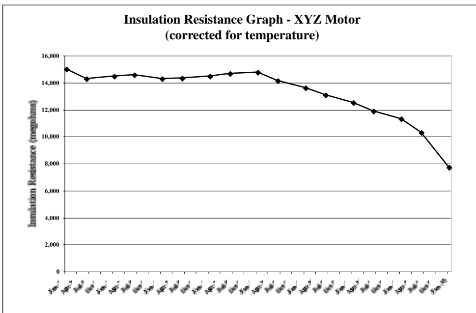
Figure 21: Insulation Resistance Graph Corrected for Temperature
