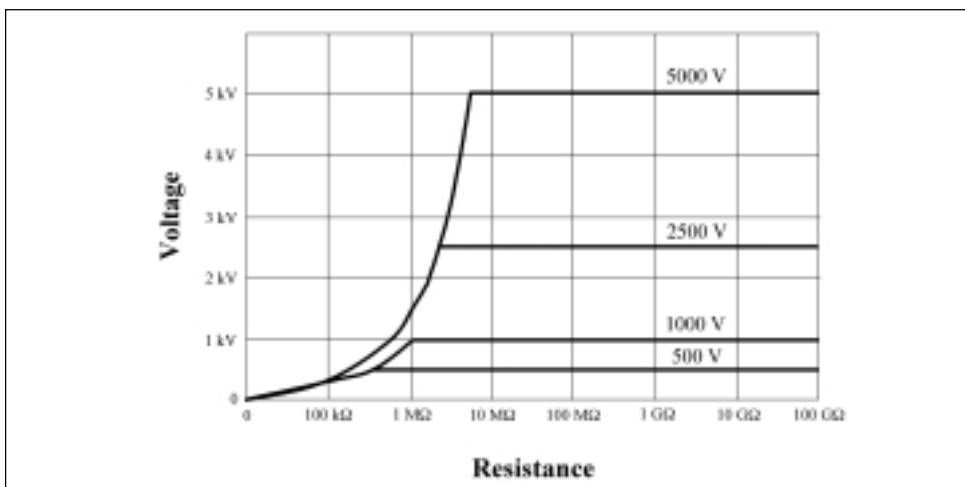
Figure 9: Good Load Curve
