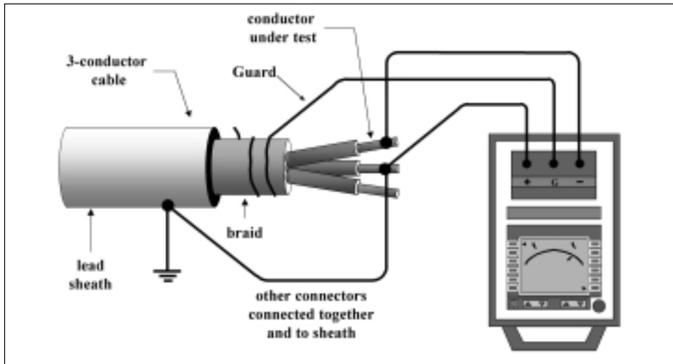
Figure 18: Use of the Guard Terminal on a Power Cable
