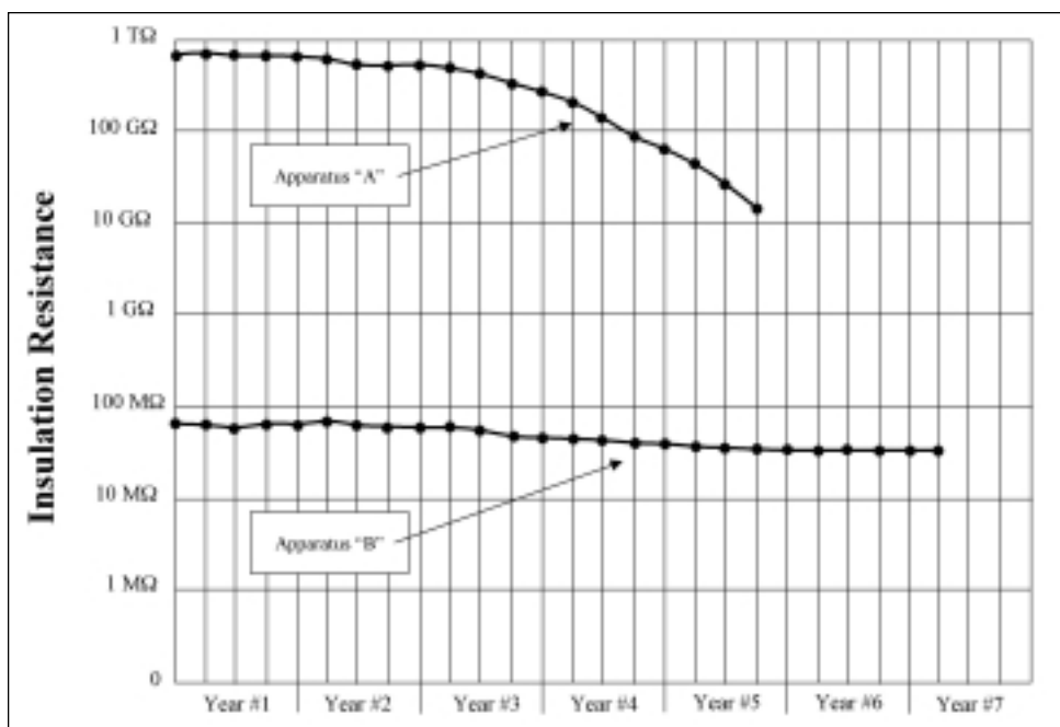
Figure 12: Comparison of Trended Test Results
