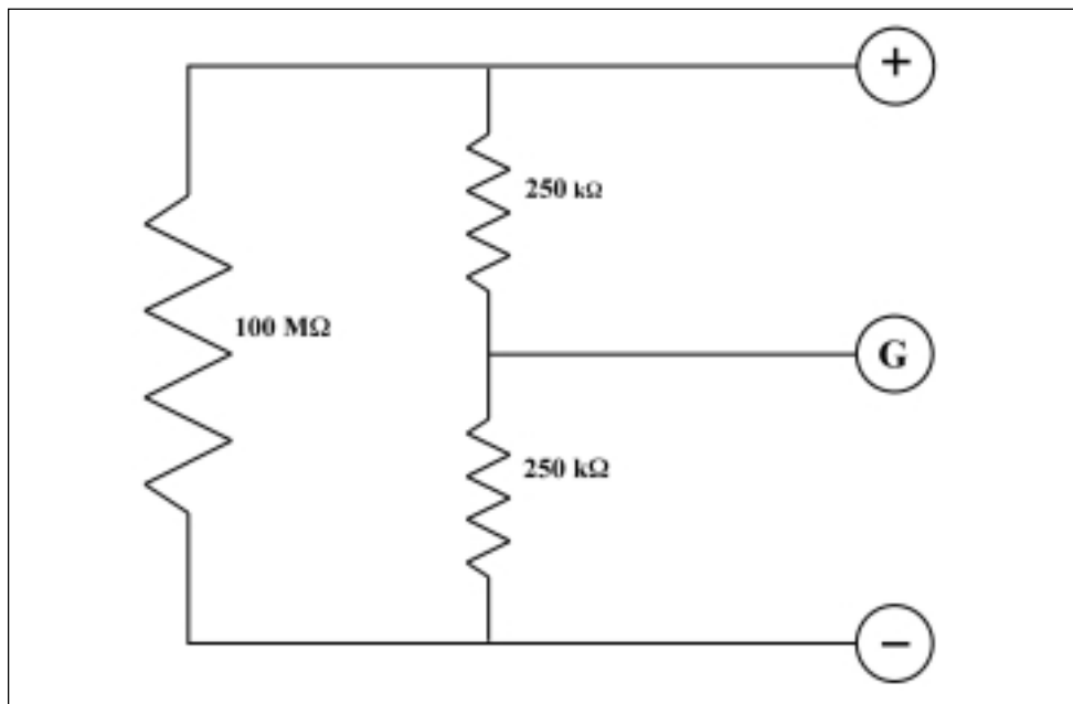
Figure 19: Guard Terminal Diagram
