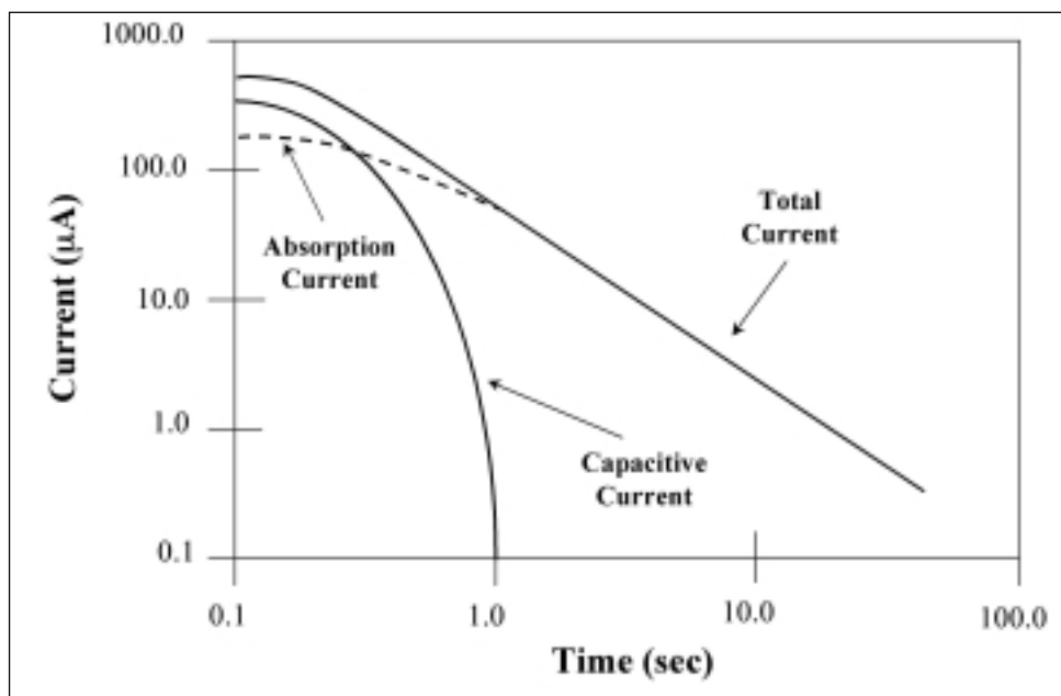
Figure 17: Reabsorption Currents
