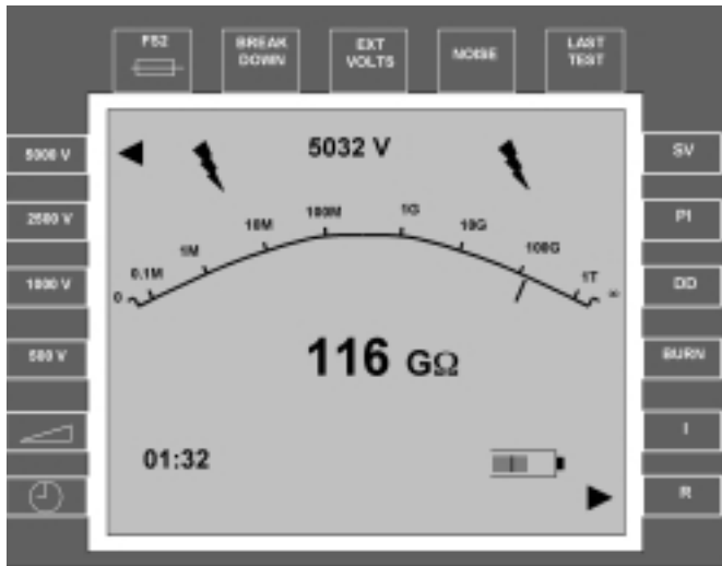
Figure 8: MEGGER BM25 Display
