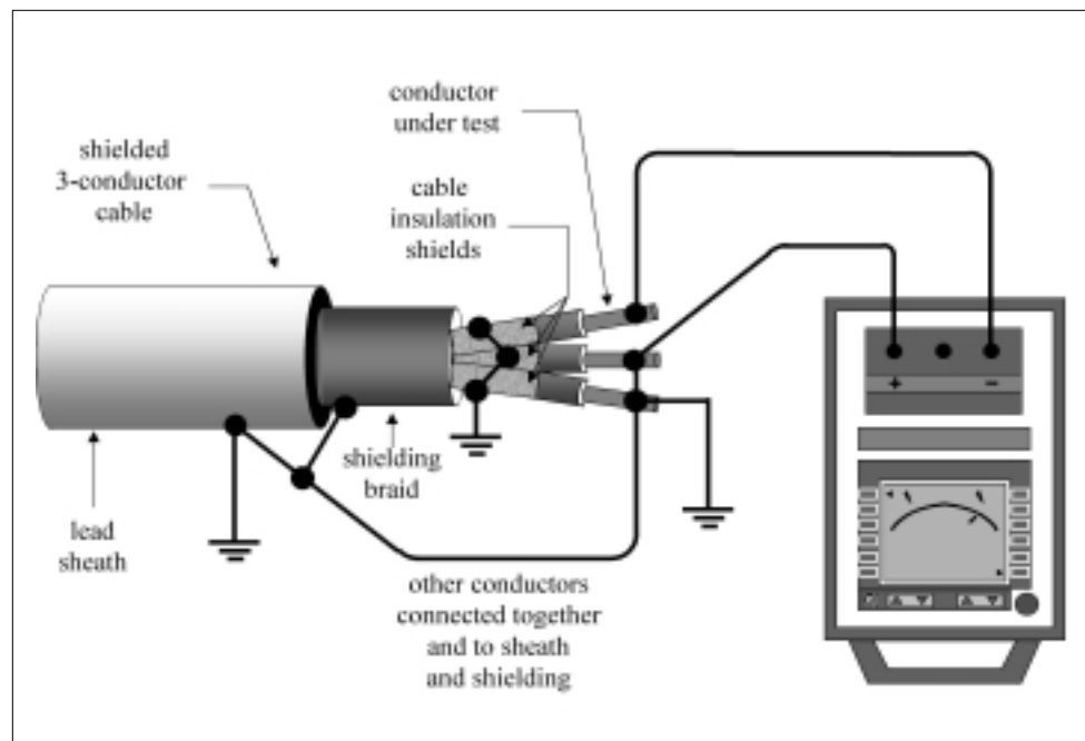
Figure 4: Connection to a Shielded Power Cable
