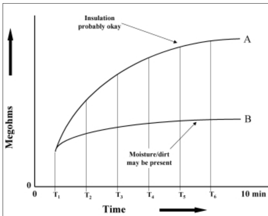
Figure 13: Time Resistance Test Graph
